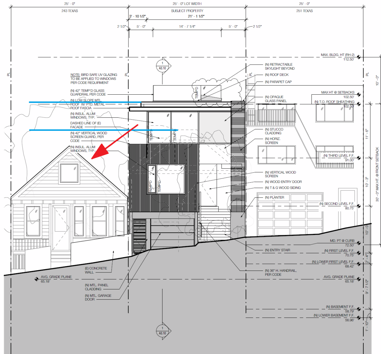
1 PROPOSED WEST ELEVATION SCALE: 3/16" = 1'-0"
