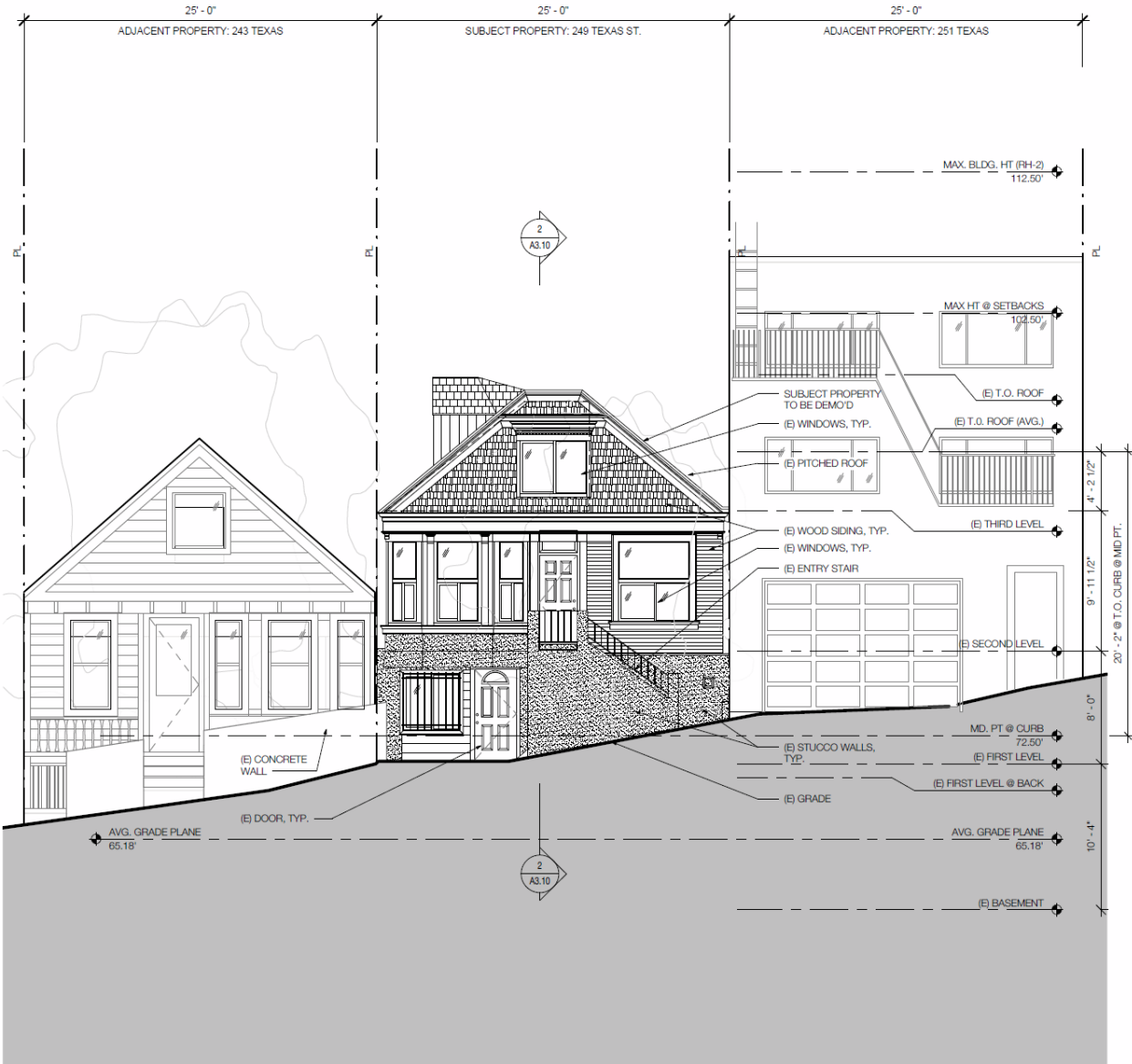
2 (E) WEST ELEVATION SCALE: 3/16" = 1'-0"
