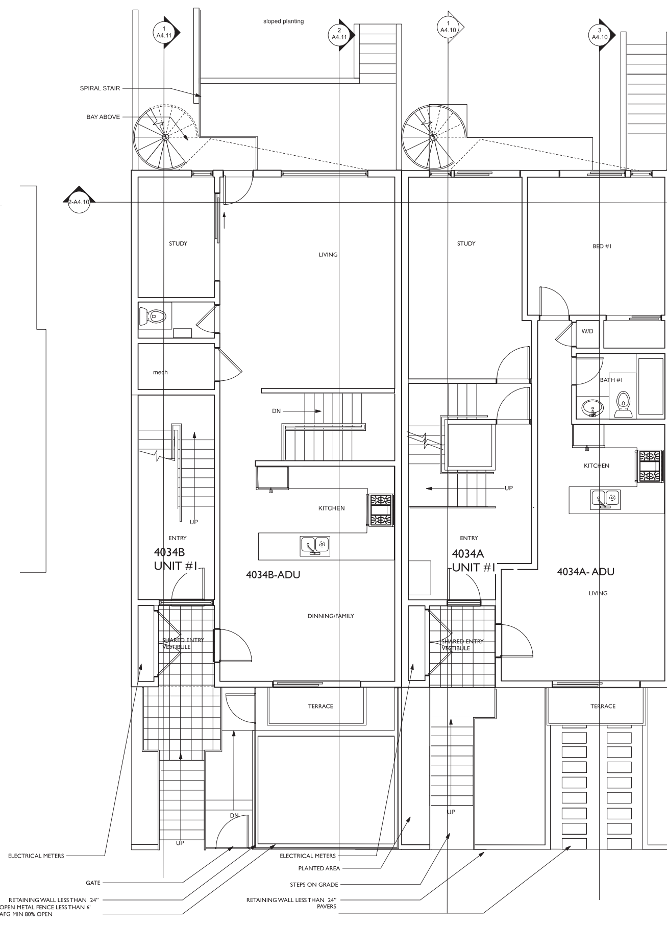
2 FIRST FLOOR 1/4"=1'-0"
