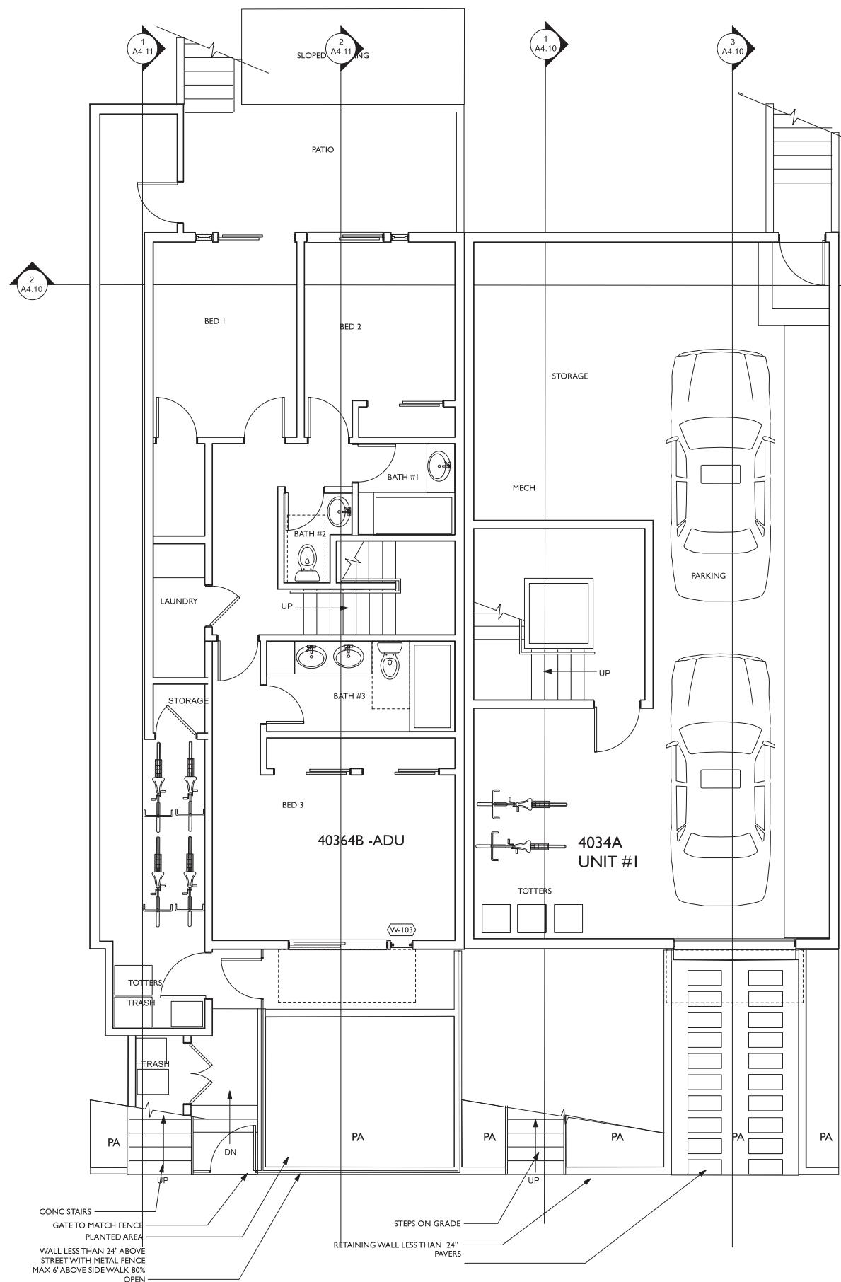
1 BASEMENT LEVEL 1/4"=1'-0"
