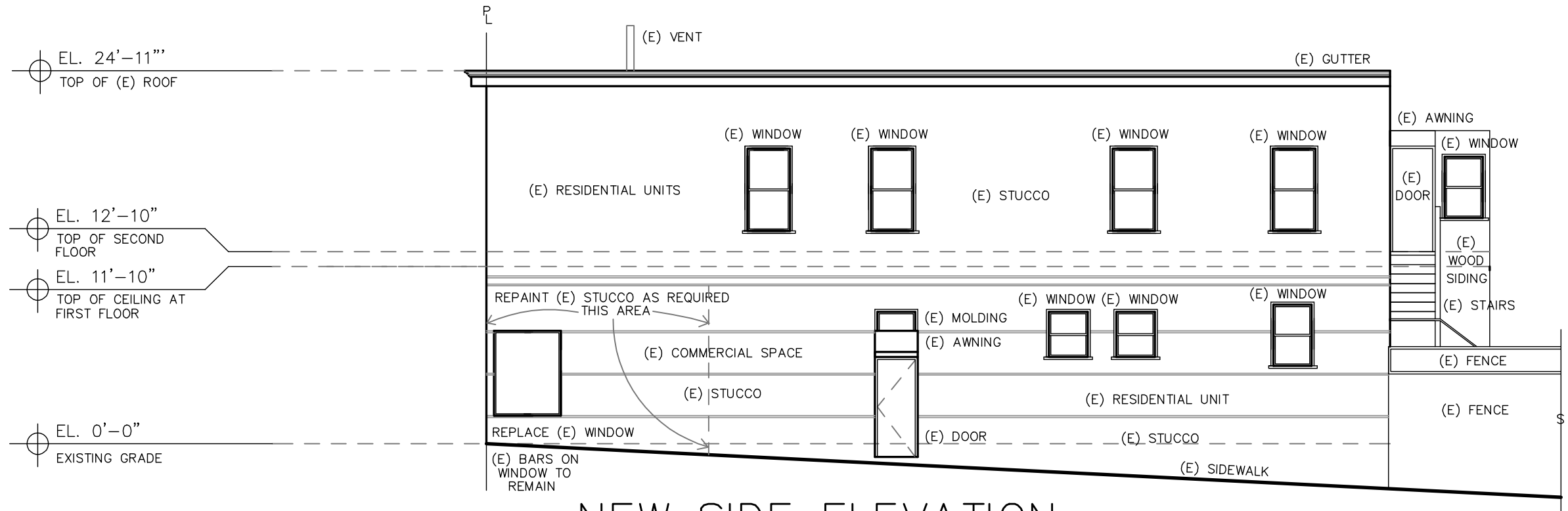
NEW SIDE ELEVATION
