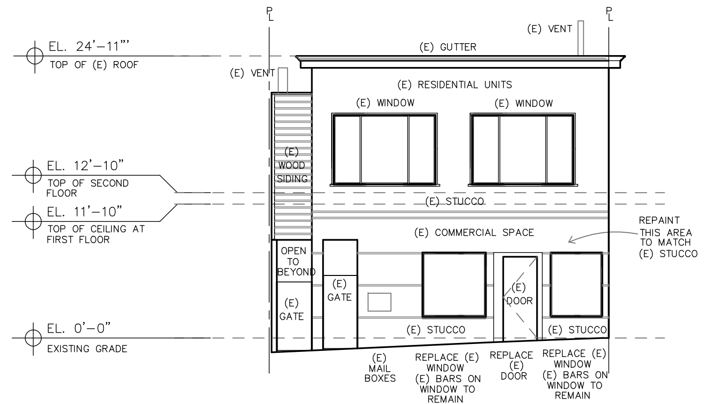
NEW FRONT ELEVATION
