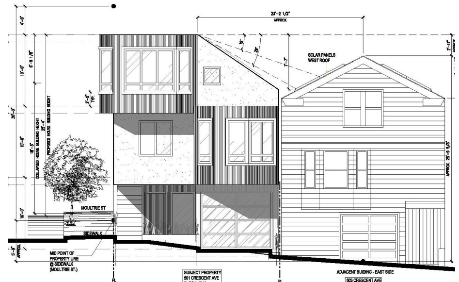
2 (N) SOUTH ELEVATION SCALE: 1/4" = 1'-0"
