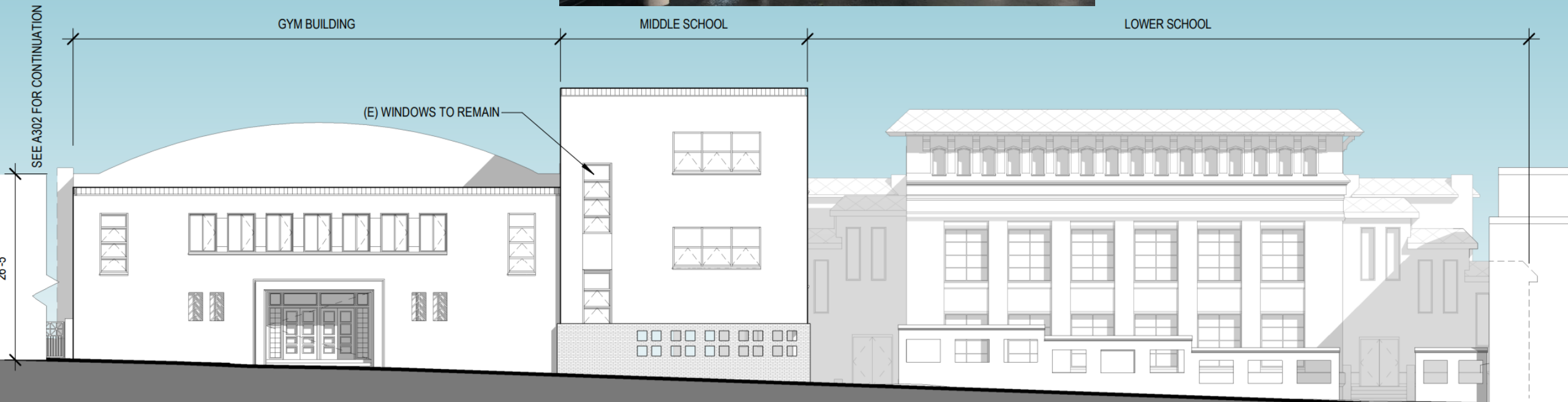
SOUTH ELEVATION - Existing
