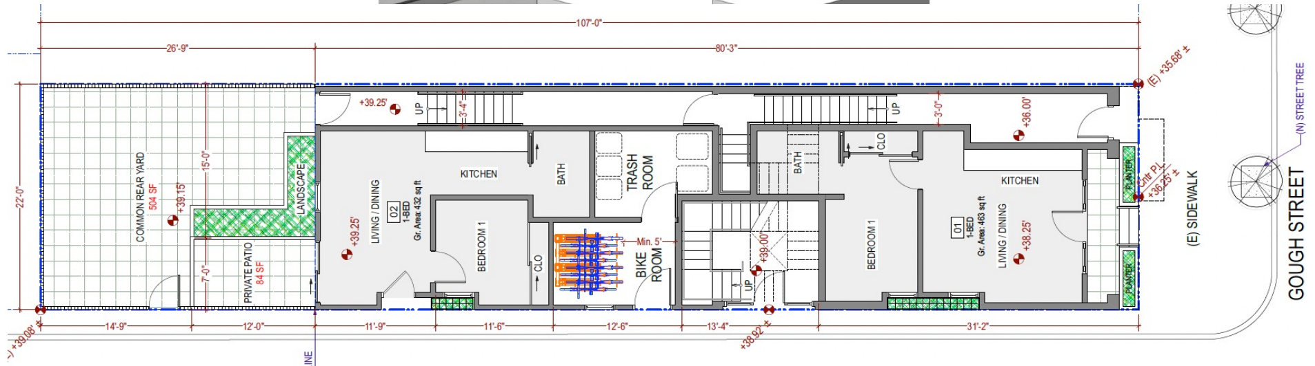
Proposed 1st Floor Plan
